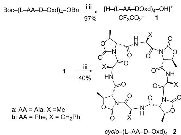
Scheme 1. Synthesis of 2a,b . Reagents and conditions: (i) H 2 , Pd/C (10%), MeOH, room temp., 12 h; (ii) TFA (18 equiv.), dry CH 2 Cl 2 , room temp., 4 h; (iii) HATU (1.1 equiv.), TEA (3 equiv.), dry CH 3 CN, room temp., 45 min.
