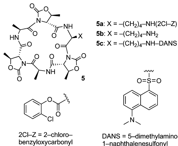
Figure 3. Chemical structure of the cyclic pseudopeptides 5a–c .
