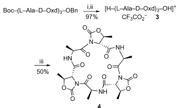
Scheme 2. Synthesis of 4 . Reagents and conditions: (i) \text{H}_2 , Pd/C (10%), MeOH, room temp., 12 h; (ii) TFA (18 equiv.), dry \text{CH}_2\text{Cl}_2 , room temp., 4 h; (iii) HATU (1.1 equiv.), TEA (3 equiv.), dry \text{CH}_3\text{CN} , room temp., 45 min.
