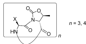
Figure 1. General chemical structure of the cyclic pseudopeptides reported in this study; X is a general side-chain.
