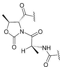
Figure 2. Preferred conformation for an L-AA-D-Oxd unit with the preferential trans conformation of the imide moiety, which accounts for the anomalous chemical shift of the amino acid CH α proton.
