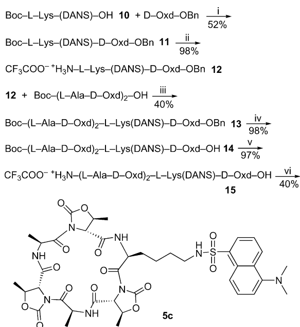
Scheme 4. Synthesis of 5c . Reagents and conditions: (i) HBTU (1 equiv.), DBU (2 equiv.), dry CH 3 CN, room temp., 3 h; (ii) TFA (18 equiv.), dry CH 2 Cl 2 , room temp., 3 h; (iii) HATU (1 equiv.), TEA (3 equiv.), dry CH 3 CN, room temp., 2 h; (iv) H 2 , Pd/C (10%), MeOH, room temp., 2 h; (v) TFA (18 equiv.), dry CH 2 Cl 2 , room temp., 3 h; (vi) HATU (1 equiv.), TEA (3 equiv.), room temp., 45 min.
