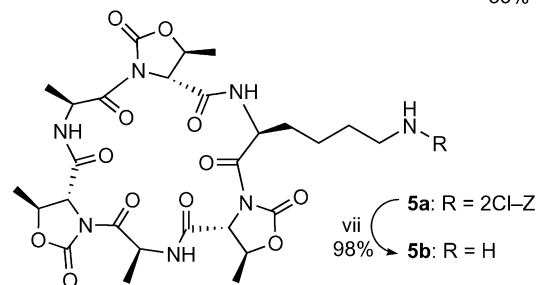
Scheme 3. Synthesis of 5b . Reagents and conditions: (i) HBTU (1 equiv.), DBU (2 equiv.), dry \text{CH}_3\text{CN} , room temp., 45 min; (ii) TFA (18 equiv.), dry \text{CH}_2\text{Cl}_2 , room temp., 3 h; (iii) HBTU (1 equiv.), TEA (3 equiv.), dry \text{CH}_3\text{CN} , room temp., 45 min; (iv) \text{H}_2 , Pd/C (10%), AcOEt, room temp., 2 h; (v) TFA (18 equiv.) dry \text{CH}_2\text{Cl}_2 , room temp., 4 h; (vi) HATU (1 equiv.), TEA (3 equiv.), room temp., 45 min; (vii) \text{H}_2 , Pd/C (10%), MeOH, room temp., 12 h.
